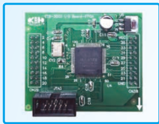
FPGA Board
