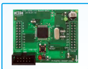
MCU Board
